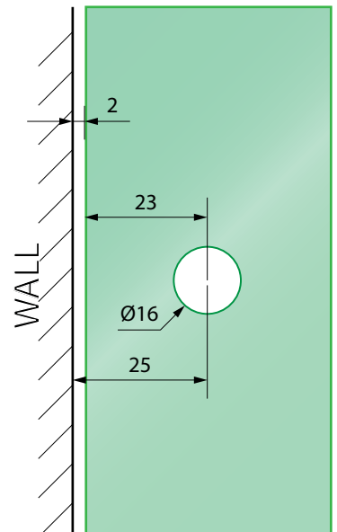
GLASS HOLE DETAIL
